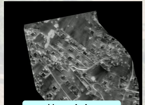
Mosaicing
