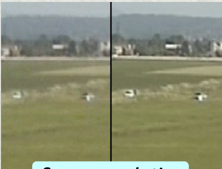
Super-resolution
